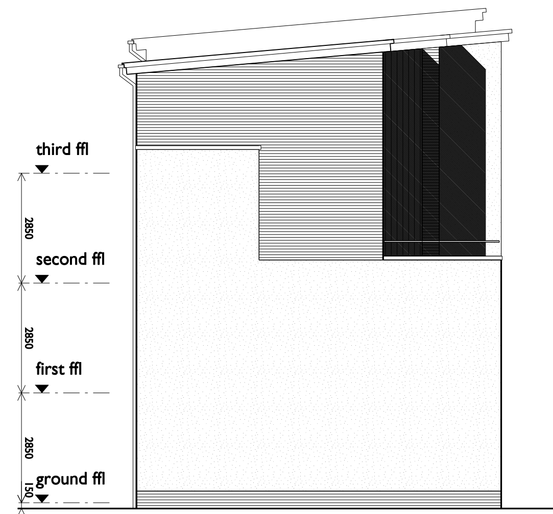
BLOCK Hiii SOUTH ELEVATION
